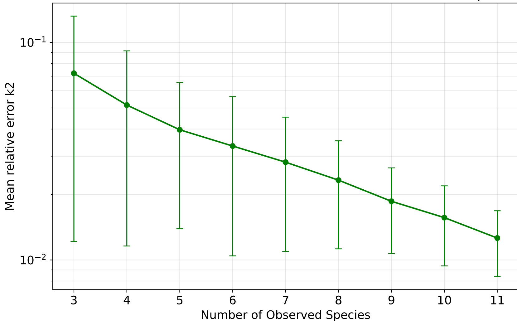
30, 30, 30 — Mean relative error k2 vs number of observed species
